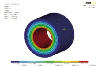
Rubber Stress / Strain Analysis
