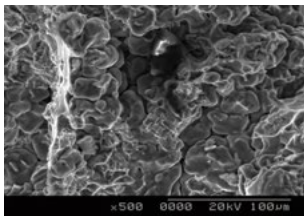
Microstructure Inspection of BaekSan Propeller
