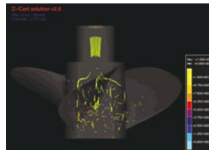
Solidification simulation
