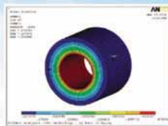
Rubber Stress / Strain Analysis
