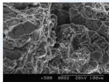
Unstable Microstructure
