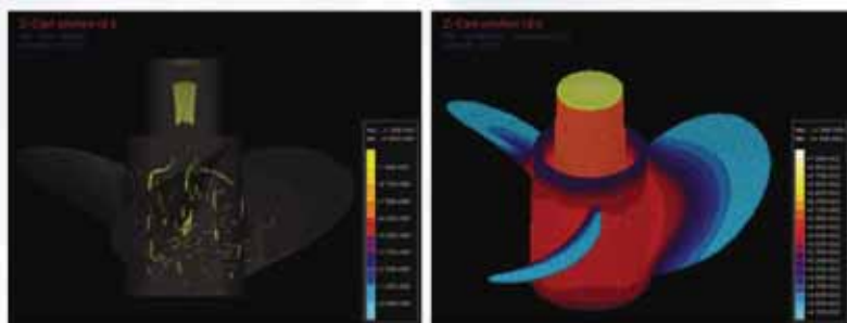
Solidification simulation
